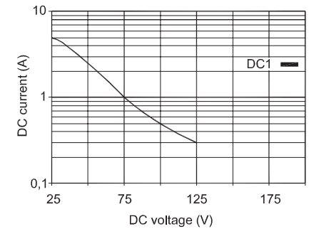
FIG. 2 MAX. DC BREAKING CAPACITY
